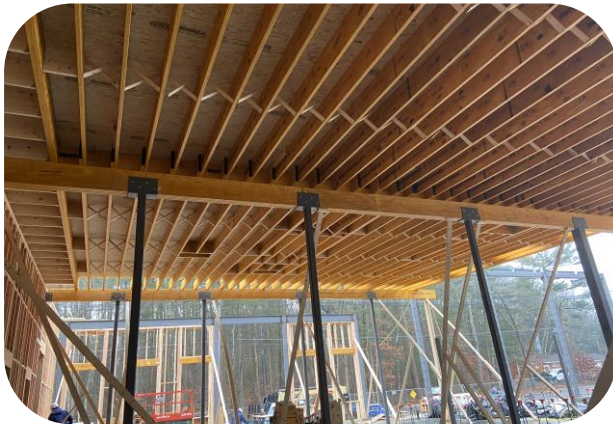
LVL joists installed on east side of building
