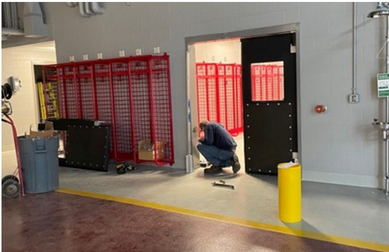
Door installation
